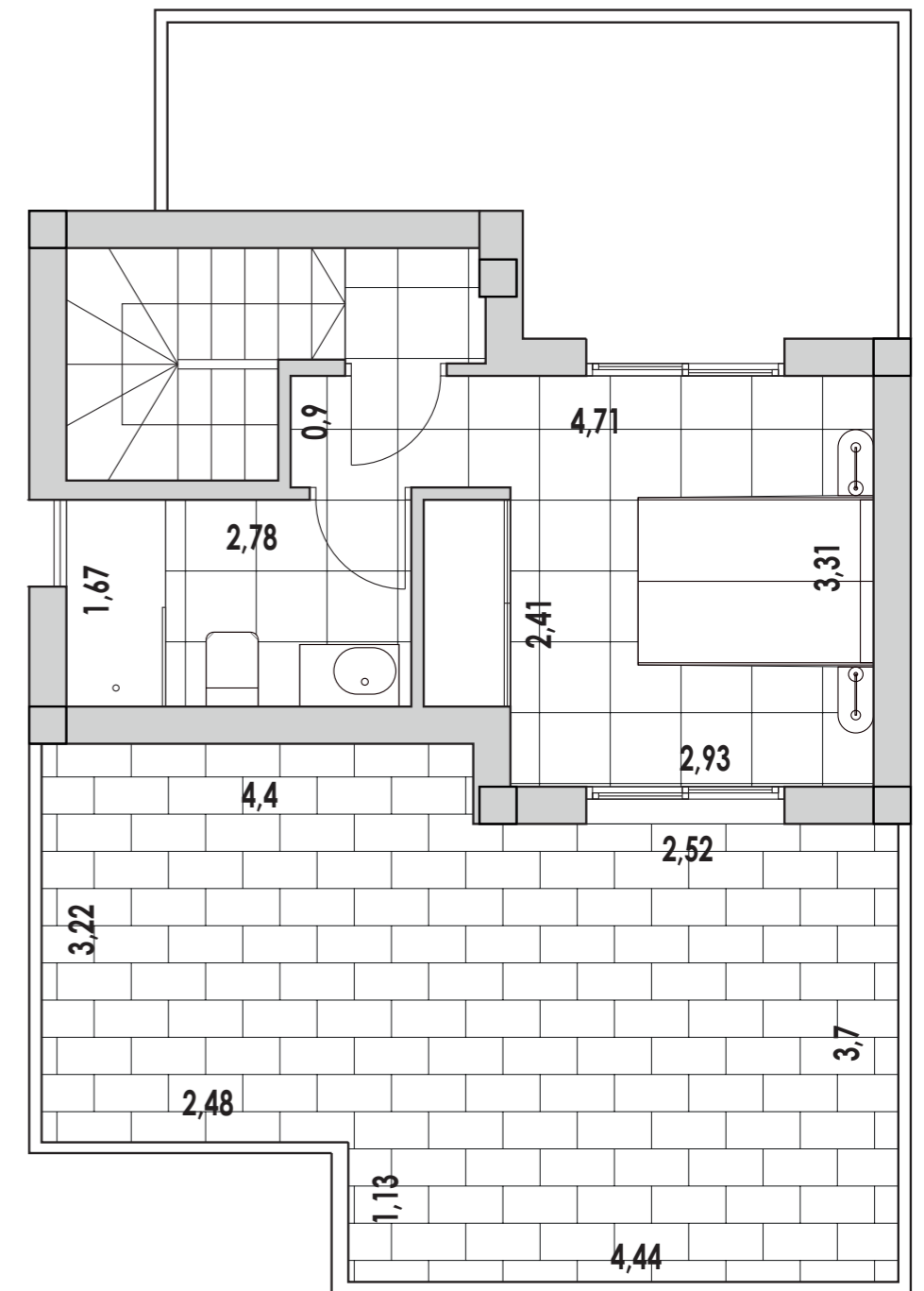
First floor
