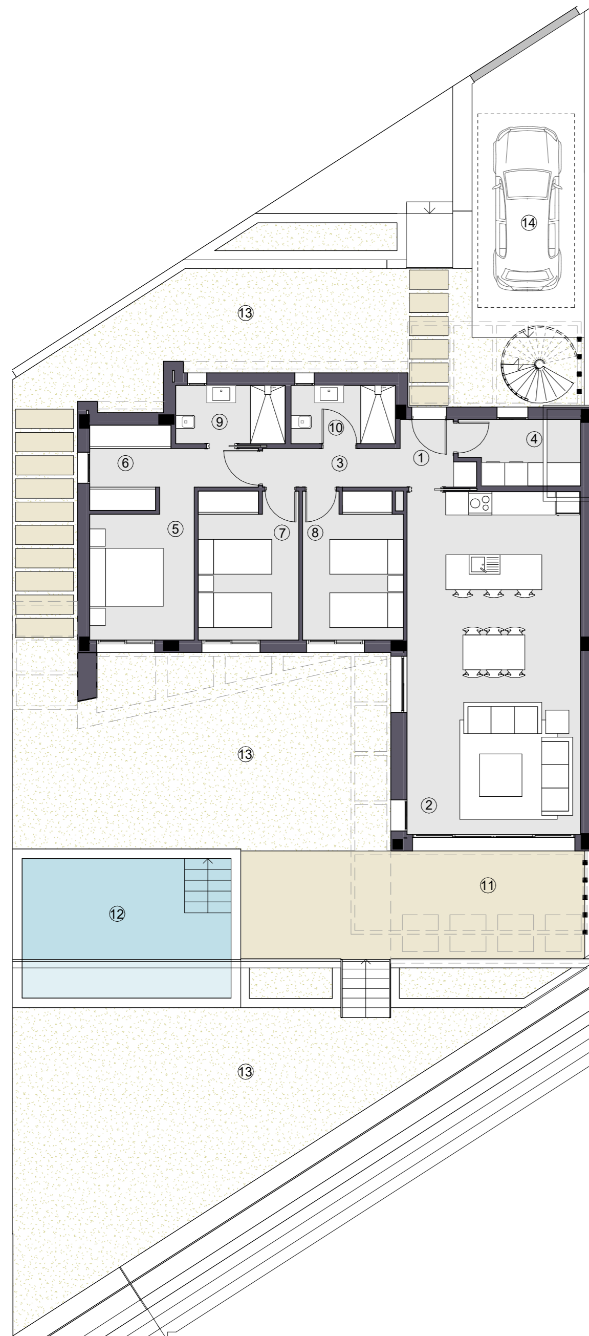
PLANTA BAJA / GROUND FLOOR
